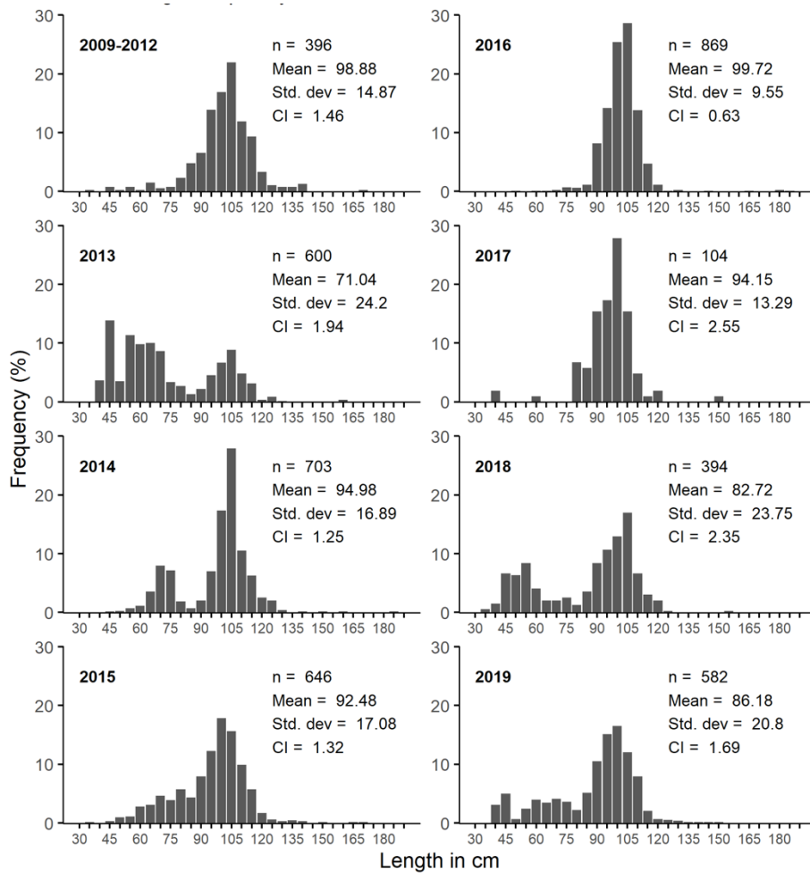
Figure 62. Length-frequency data of jurel aggregated across all years (2009-2019) and depth categories; plotted by time period.
