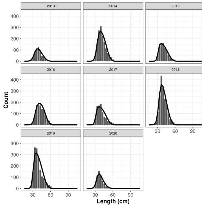
Figure 44. Initial LBSPR assessment of pargo amarillo using size composition of the catch data aggregated fishing areas and depths and fitted by year, assuming L_{50} = 37 cm & L_m/L_\infty = 0.72 to infer L_\infty = 51 cm. Plots of the size composition data analysed (black bars) and the LBSPR modelled fit to those data (black line).
