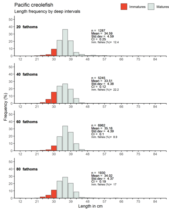
Figure 48. Length-frequency data aggregated across all years (2009-2019) and all fishing locations plotted by depth category. Size at maturity according to Rivera-Comacho et al. (2015) indicated by darker colouring.
