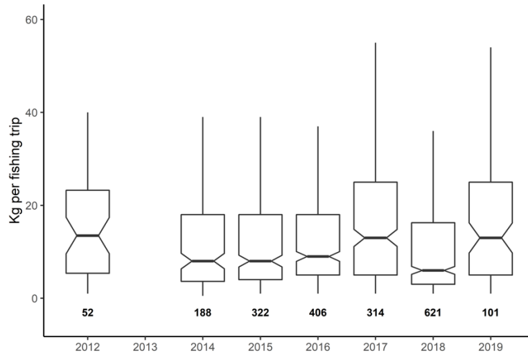
Figure 23. Catch-Per-Unit-Effort data for cabrilla sardinera aggregated across all depth categories and fishing areas, plotted annually. Bold values mark sample size for each year, black horizontal bars indicate medians with 95% confidence intervals indicated by notches, boxes indicate interquartile range (0.25 – 0.75) and vertical lines the range.
