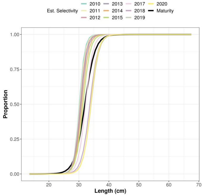
Figure 107. Results of initial LBSPR of verdillo using size composition of the catch data aggregated fishing areas and depths and fitted by year. Plots of assumed size of maturity ogive (black) and estimated size of selectivity (coloured).
