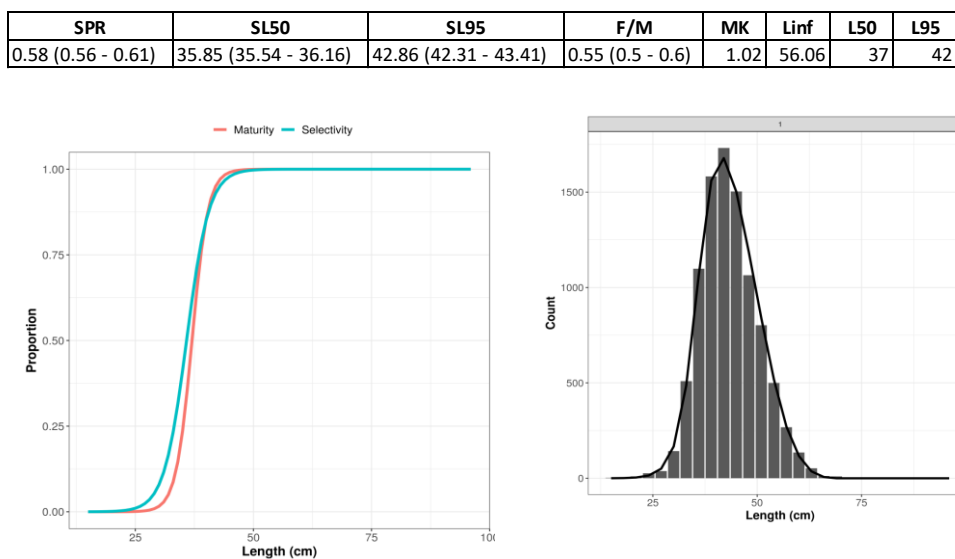
Figure 84. Initial LBSPR assessment using size composition of the catch data aggregated across all years, fishing areas and depths. The table shows derived estimates of spawning ratio potential (SPR) and the size of 50% and 95% selectivity (SL50 & SL95) and relative fishing pressure (F/M). The estimated 95% confidence intervals around these mean estimates are shown in brackets. The input parameters assumed are indicated to the right; life history ratio M/K, asymptotic size (Linf), size at 50% and 95% maturity (L50 & L95). The left-hand panel presents plots of assumed size of maturity ogive (red) and the estimate size of selectivity (blue). The right-hand panel plots the size composition data analysed (black bars) and the LBSPR modelled fit to those data.
