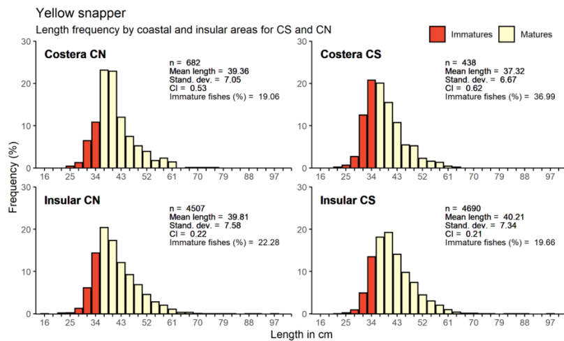
Figure 31. Length-frequency data of pargo amarillo aggregated across all years (2009-2019); plotted by coastal (costera) and offshore (Insular) in the north and south of El Corredor. Size at maturity according to Barbosa-Ortega et al. (2014) indicated by darker colouring.
