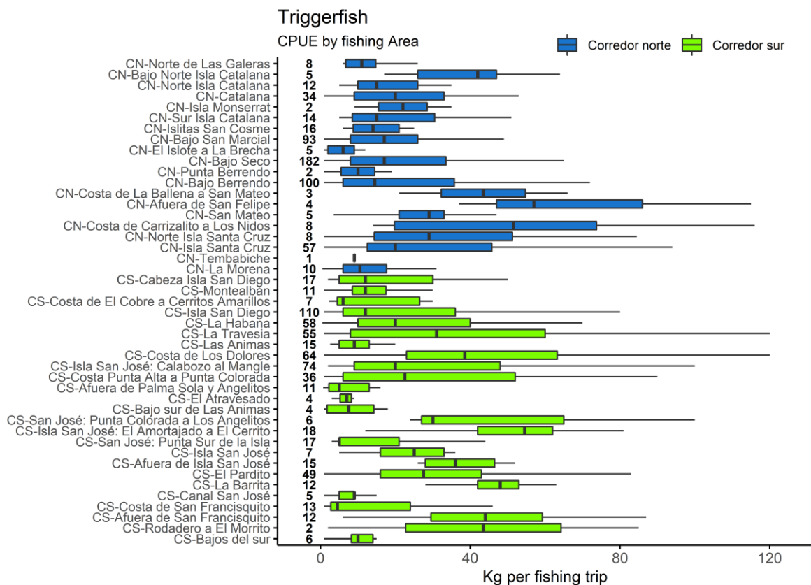
Figure 5. Percentile catch-per-unit-effort data for cochito aggregated across all years (2009-2019) and depth categories, plotted by fishing area sorted north to south. Bold values mark sample size for each area, black bars indicate median, coloured bars indicate interquartile range (0.25 – 0.75), horizontal lines the range. Confidence intervals cannot be estimated due to low record numbers for most fishing areas.
