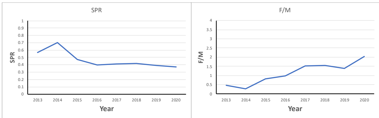
Figure 16. Initial LBSPR assessment of cochito using size composition of the catch data aggregated fishing areas and depths and fitted by year, assuming Monocanthidae LHR ( M/k=1.47 ; L_m/L_\infty = 0.647 ) and L_m = 33.5 cm as estimated for El Corredor and thus L_\infty = 52 cm. Plots of the estimate trend in SPR (left) and relative fishing pressure (F/M) by year (right).
