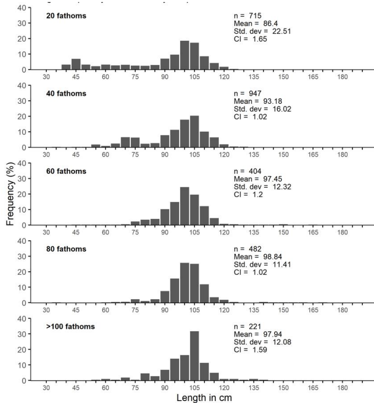
Figure 61. Length-frequency data aggregated across all years (2009-2019) and all fishing locations plotted by depth category.
