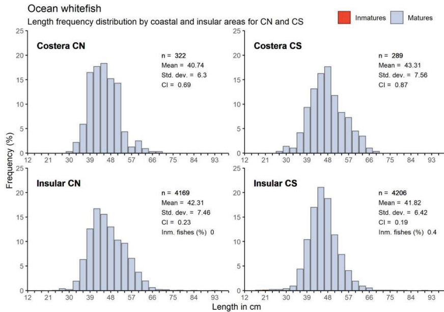
Figure 76. [CA11]Length-frequency data for pierna aggregated across all years (2009-2019); plotted by coastal (costera) and offshore (Insular) in the north and south of El Corredor. Size at maturity according to Ramirez-Luna (2010).
