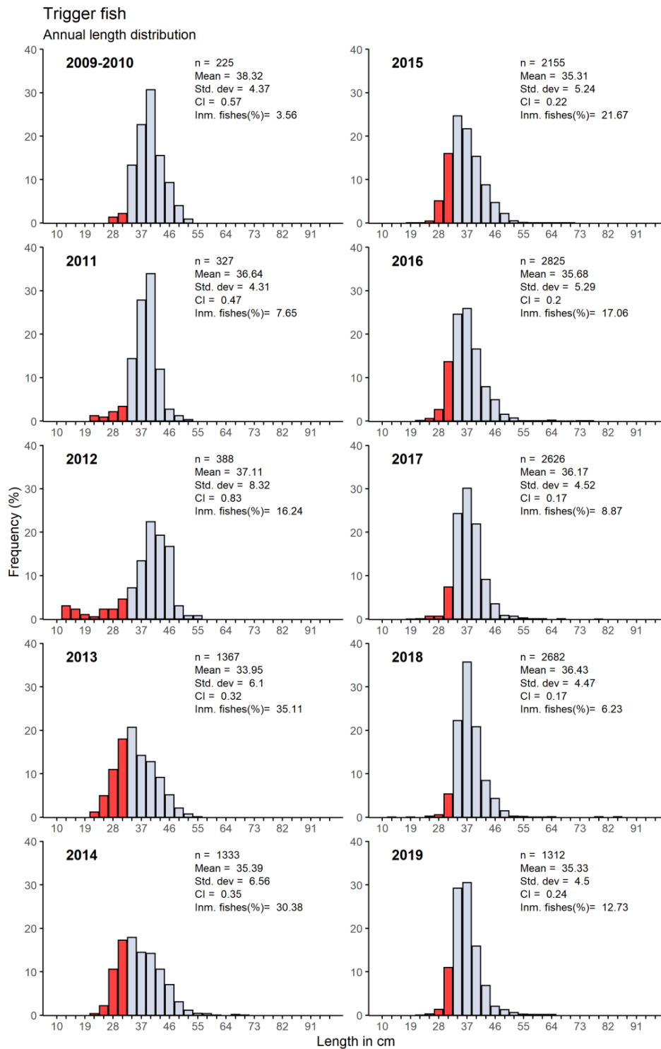
Figure 4. Length-frequency data for cochito aggregated across fishing areas and depth categories; plotted by year/s. Size at maturity according to Camacho Mondragon et al. (2019) indicated by darker colouring.
