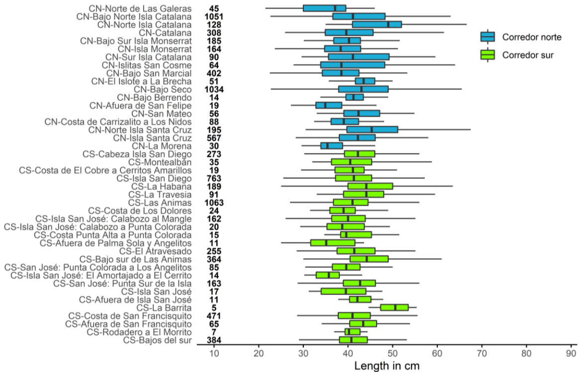
Figure 75. Percentile length-frequency data for pierna aggregated across all years (2009-2019) and depth categories; plotted by fishing areas sorted north to south. Bold values mark sample size for each area, black bars indicate median, coloured bars indicate interquartile range (0.25 – 0.75), horizontal lines the range. Confidence intervals cannot be estimated due to low record numbers for most fishing areas.
