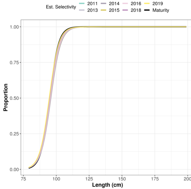
Figure 69. Initial annual LBSPR assessment of jurel using size composition of the catch aggregated across fishing areas from \geq 40 fathoms and truncated at 75 cm; assuming L_{\infty} = 153 cm & L_m/L_{\infty} = 0.72 to infer L_{50} = 95 cm. Plots of assumed size of maturity ogive (black) and estimated size of selectivity (coloured).
