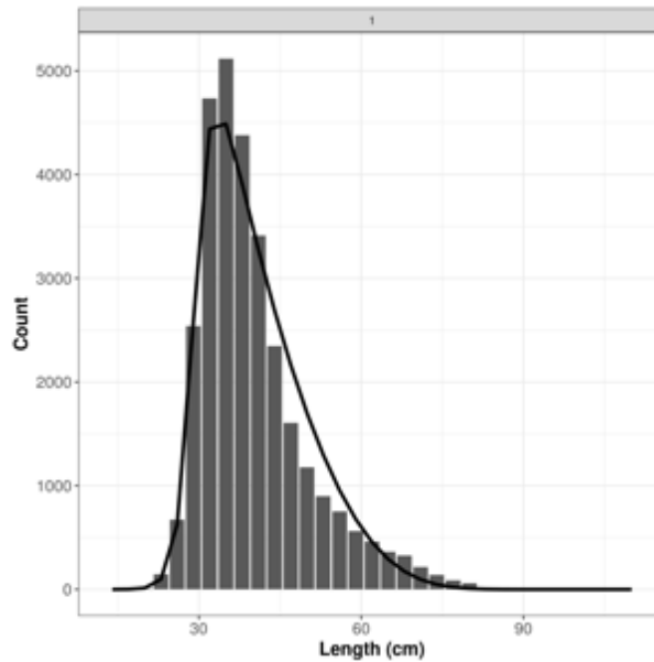
Figure 99. LBSPR fitting to the huachinango catch size composition data aggregated across all years, fishing locations and depths categories.
