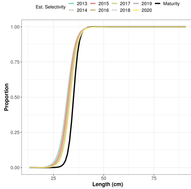
Figure 11. Results of initial LBSPR of cochito using size composition of the catch data aggregated fishing areas and depths and fitted by year, assuming L_{\infty} = 56 cm and L_{50} = 35 cm. Plots of assumed size of maturity ogive (black) and estimated size of selectivity (coloured).
