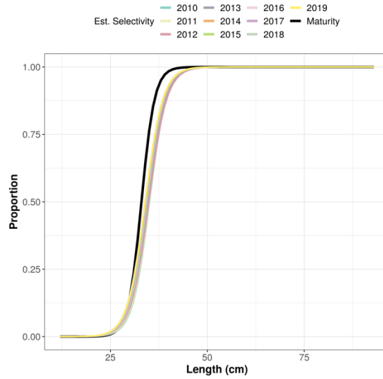
Figure 56. Results of initial LBSPR assessment of cadernal using size composition of the catch data aggregated fishing areas and depths and fitted by year. Plots of assumed size of maturity ogive (black) and estimated size of selectivity (coloured).
