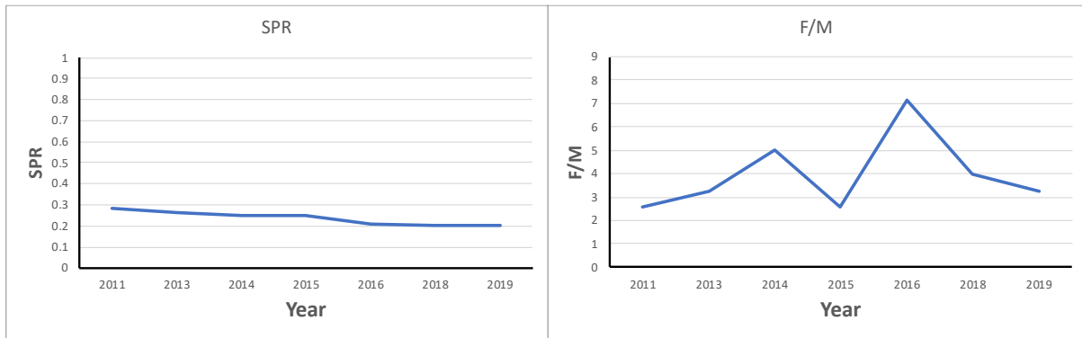
Figure 74. Annual LBSPR assessment of jurel using size composition of the catch aggregated across fishing areas from \geq 40 fathoms and truncated at 75 cm; assuming L_{50} = 90 cm & L_m/L_\infty = 0.72 to infer L_\infty = 145 cm. Plots of the estimate trend in SPR (left) and relative fishing pressure (F/M) by year (right).
