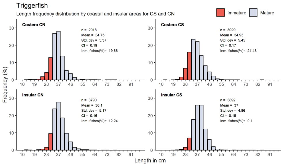
Figure 2. Length-frequency data for cochito aggregated across all years (2009-2019); plotted by coastal (costera) and offshore (Insular) in the north and south of El Corredor. Size at maturity (33.8 cm) according to Camacho Mondragon et al. (2019) indicated by darker colouring.
