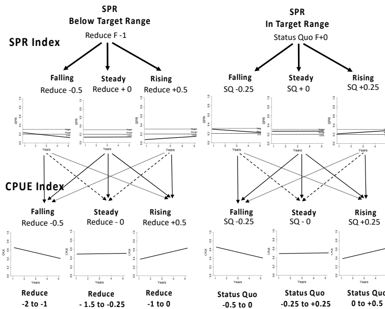
Figure 117. Model of Harvest Control Rule adapted for fisheries with dome-shaped selectivity.
