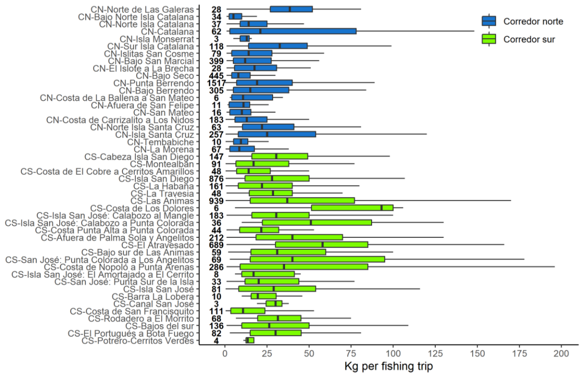
Figure 94. Percentile catch-per-unit-effort data for huachinango aggregated across all years (2009-2019) and depth categories, plotted by fishing area sorted north to south. Bold values mark sample size for each area, black bars indicate median, coloured bars indicate interquartile range (0.25 – 0.75), horizontal lines the range. Confidence intervals cannot be estimated due to low record numbers for most fishing areas.
