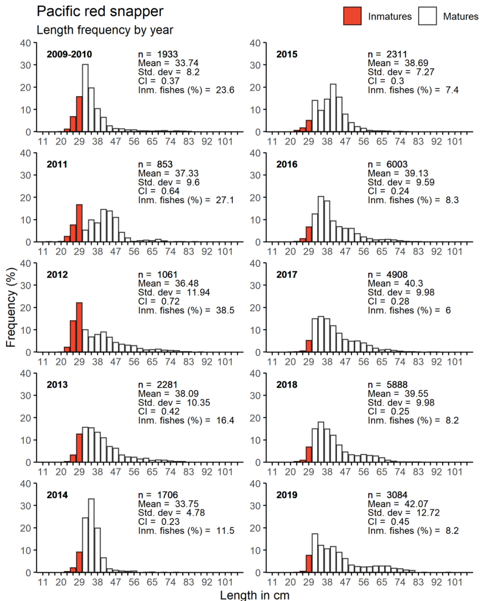
Figure 91. Length-frequency data for huachinango aggregated across all fishing areas and depth categories; plotted by time period. Size at maturity according to Barbosa-Ortega et al. (2014) indicated by darker colouring.
