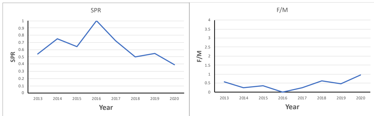
Figure 45. Initial LBSPR assessment of pargo amarillo using size composition of the catch data aggregated fishing areas and depths and fitted by year, assuming L_{50} = 37 cm & L_m/L_\infty = 0.72 to infer L_\infty = 51 cm. Plots of the estimate trend in SPR (left) and relative fishing pressure (F/M) by year (right).
