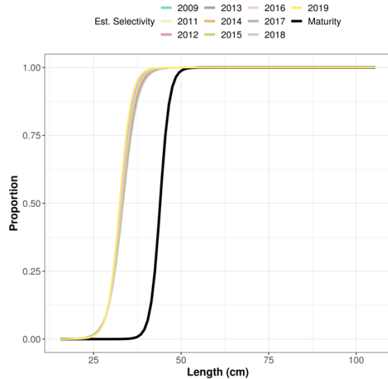
Figure 40. Results of initial LBSPR of pargo amarillo using size composition of the catch data aggregated fishing areas and depths and fitted by year, assuming L_{\infty} = 61 cm & L_m/L_{\infty} = 0.72 to infer L_{50} = 44 cm. Plots of assumed size of maturity ogive (black) and estimated size of selectivity (coloured).
