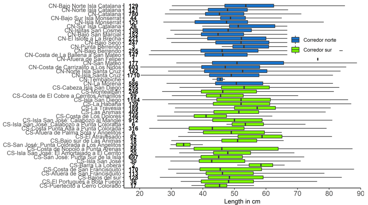
Figure 17. Percentile length-frequency data for cabrilla sardinera aggregated across all years (2009-2019) and depth categories; plotted by fishing areas sorted north to south. Bold values mark sample size for each area, black bars indicate median, coloured bars indicate interquartile range (0.25 – 0.75), horizontal lines the range. Confidence intervals cannot be estimated due to low record numbers for most fishing areas.
