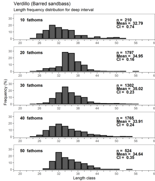
Figure 102. Verdillo length-frequency data 2017-20 by 10 fathom depth categories illustrating that the smaller size compositions are most prevalent in <10 fathoms.
