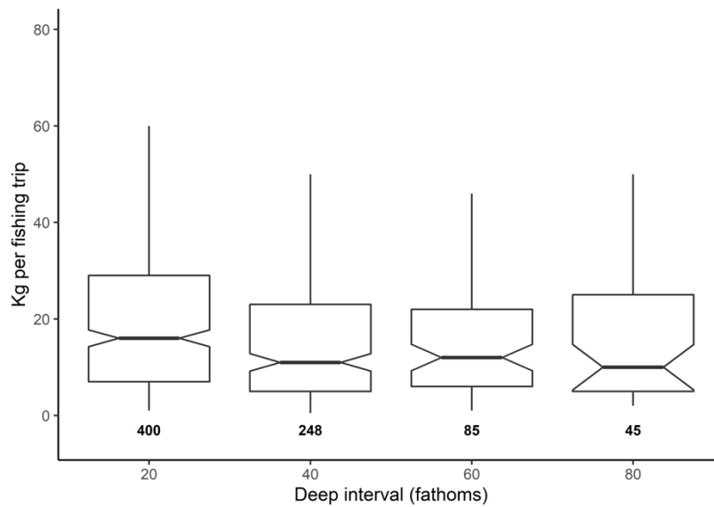
Figure 22. Catch-Per-Unit-Effort data for cabrilla sardinera aggregated across all years (2009-2019) and fishing locations; plotted by depth category. Bold values mark sample size for each year, black horizontal bars indicate medians with 95% confidence intervals indicated by notches, boxes indicate interquartile range (0.25 – 0.75) and vertical lines the range.
