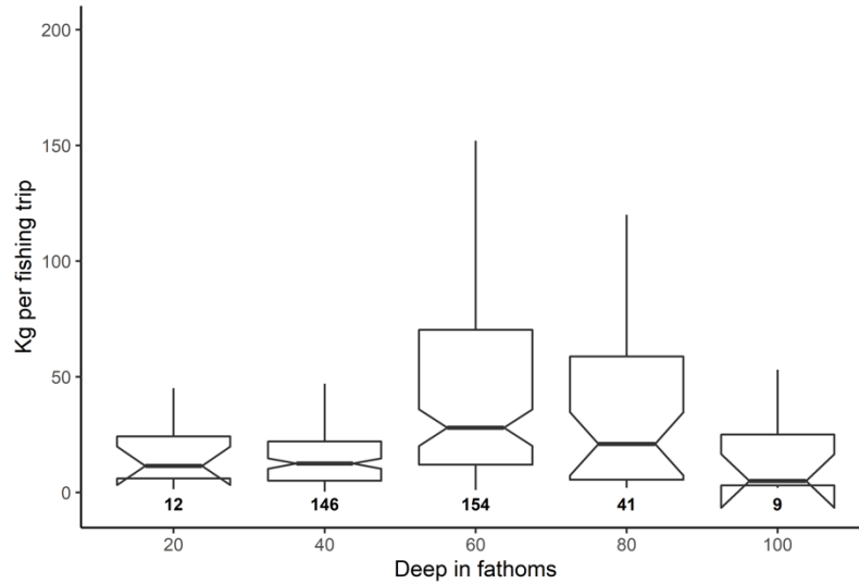
Figure 80. Catch-Per-Unit-Effort data for pierna aggregated across all years (2009-2019) and fishing locations; plotted by depth category. Bold values mark sample size for depth category, black horizontal bars indicate medians with 95% confidence intervals indicated by notches, boxes indicate interquartile range (0.25 – 0.75) and vertical lines the range. The unusual shape of the last boxplot indicates the low sample size.
