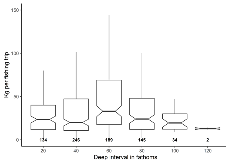
Figure 64. Catch-Per-Unit-Effort data for jurel aggregated across all years (2009-2019) and fishing locations; plotted by depth category. Bold values mark sample size for each year, black horizontal bars indicate medians with 95% confidence intervals indicated by notches, boxes indicate interquartile range (0.25 – 0.75) and vertical lines the range.
