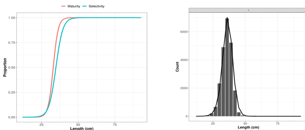
Figure 55. Initial LBSPR assessment using size composition of the catch data aggregated across all years, fishing areas and depths. The table shows derived estimates of spawning ratio potential (SPR) and the size of 50% and 95% selectivity (SL50 & SL95) and relative fishing pressure (F/M). The estimated 95% confidence intervals around these mean estimates are shown in brackets. The input parameters assumed are indicated to the right; life history ratio M/K, asymptotic size (Linf), size at 50% and 95% maturity (L50 & L95). The left-hand panel presents plots of assumed size of maturity ogive (red) and the estimate size of selectivity (blue). The right-hand panel plots the size composition data analysed (black bars) and the LBSPR modelled fit to those data.
