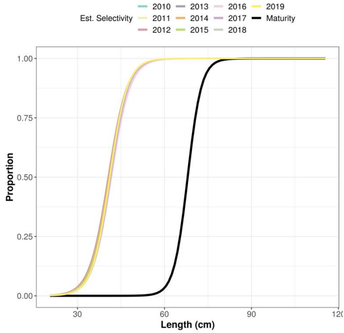
Figure 27. Results of initial LBSPR assessment of cabrilla sardinera using size composition of the catch data aggregated fishing areas and depths and fitted by year. Plots of assumed size of maturity ogive (black) and estimated size of selectivity (coloured).
