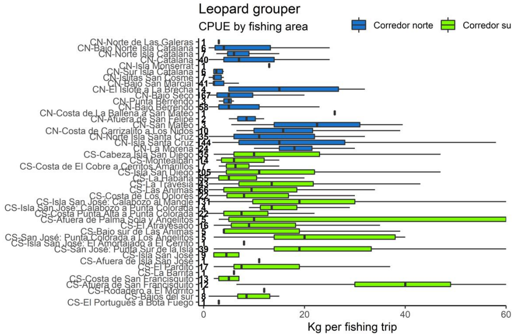
Figure 21. Percentile catch-per-unit-effort data for cabrilla sardinera aggregated across all years (2009-2019) and depth categories, plotted by fishing area sorted north to south. Bold values mark sample size for each area, black bars indicate median, coloured bars indicate interquartile range (0.25 – 0.75), horizontal lines the range. Confidence intervals cannot be estimated due to low record numbers for most fishing areas.
