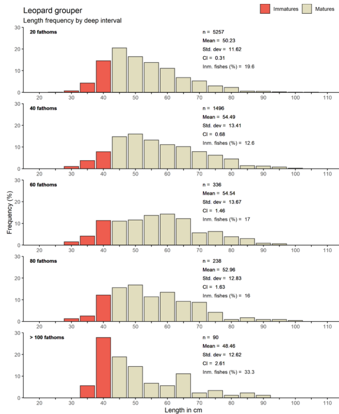
Figure 19. Length-frequency data for cabrilla sardinera aggregated across all years (2009-2019) fishing locations; plotted by depth category. Size at maturity according to Perez-Olivas et al. (2018) indicated by darker colouring.
