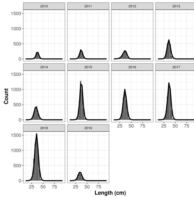
Figure 57. Initial LBSPR assessment of cadernal using size composition of the catch data aggregated fishing areas and depths and fitted by year. Plots of the size composition data analysed (black bars) and the LBSPR modelled fit to those data (black line).
