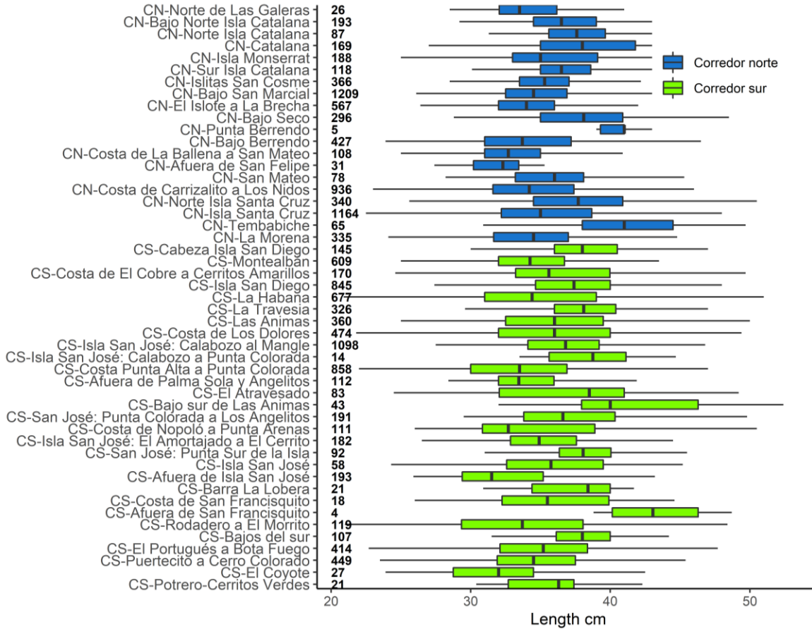
Figure 1. Percentile length-frequency data for cochito aggregated across all years (2009-2019) and depth categories; plotted by fishing areas sorted north to south. Bold values mark sample size for each area, black bars indicate median, coloured bars indicate interquartile range (0.25 – 0.75), horizontal lines the range. Confidence intervals cannot be estimated due to low record numbers for most fishing areas.
