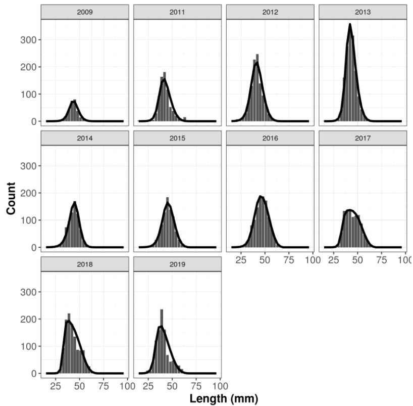
Figure 86. Initial LBSPR assessment of pierna using size composition of the catch data aggregated fishing areas and depths and fitted by year. Plots of the size composition data analysed (black bars) and the LBSPR modelled fit to those data (black line).
