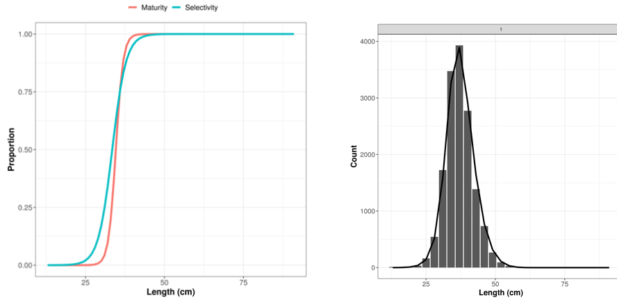
Figure 10. Initial LBSPR assessment using size composition of the catch data aggregated across all years, fishing areas and depths. The table shows derived estimates of spawning ratio potential (SPR) and the size of 50% and 95% selectivity (SL 50 & SL 95 ) and relative fishing pressure (F/M). The estimated 95% confidence intervals around these mean estimates are shown in brackets. The input parameters assumed are indicated to the right; life history ratio M/K, asymptotic size (Linf), size at 50% and 95% maturity (L 50 & L 95 ). The left-hand panel presents plots of assumed size of maturity ogive (red) and the estimate size of selectivity (blue). The right-hand panel plots the size composition data analysed (black bars) and the LBSPR modelled fit to those data.
