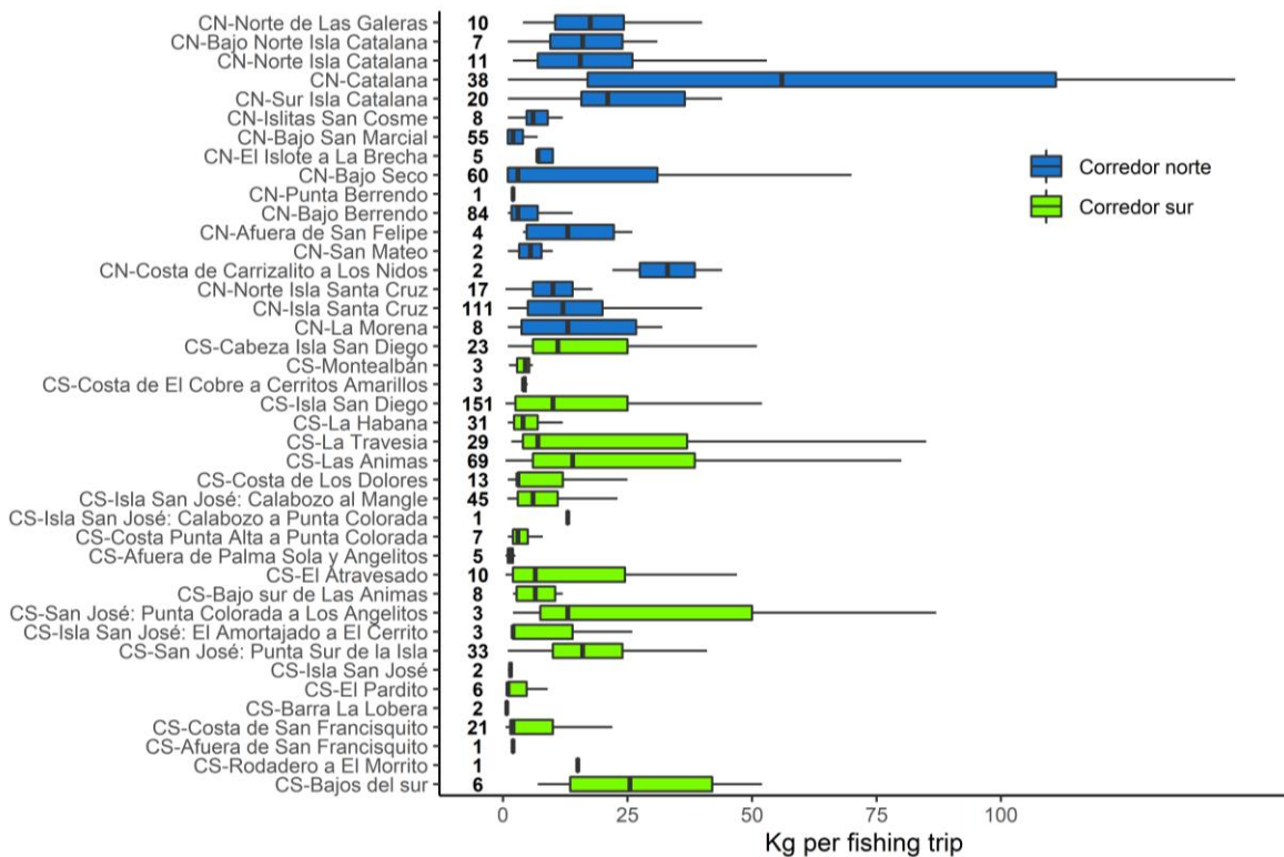
Figure 34. Percentile catch-per-unit-effort data for pargo amarillo aggregated across all years (2009-2019) and depth categories, plotted by fishing area sorted north to south. Bold values mark sample size for each area, black bars indicate median, coloured bars indicate interquartile range (0.25 – 0.75), horizontal lines the range. Confidence intervals cannot be estimated due to low record numbers for most fishing areas.
