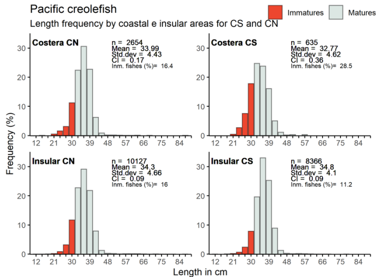
Figure 47. Length-frequency data of cadernal aggregated across all years (2009-2019); plotted by coastal (costera) and offshore (Insular) in the north and south of El Corredor. Size at maturity according to Rivera-Comacho et al. (2015) indicated by darker colouring.
