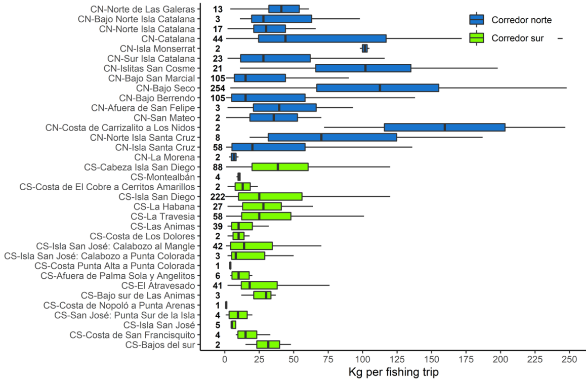
Figure 50. Percentile catch-per-unit-effort data for cadernal aggregated across all years (2009-2019) and depth categories, plotted by fishing area sorted north to south. Bold values mark sample size for each area, black bars indicate median, coloured bars indicate interquartile range (0.25 – 0.75), horizontal lines the range. Confidence intervals cannot be estimated due to low record numbers for most fishing areas.
