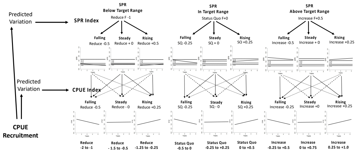
Figure 118. Model of Harvest Control Rule adapted for fisheries with periodic recruitment pulses.
