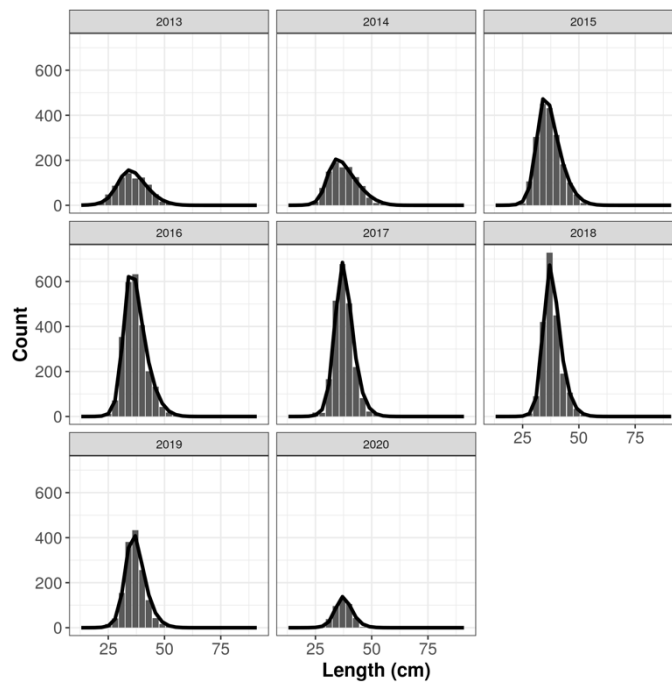
Figure 12. Initial LBSPR assessment of cochito using size composition of the catch data aggregated fishing areas and depths and fitted by year, assuming L_{\infty} = 56 cm and L_{50} = 35 cm. Plots of the size composition data analysed (black bars) and the LBSPR modelled fit to those data (black line).
