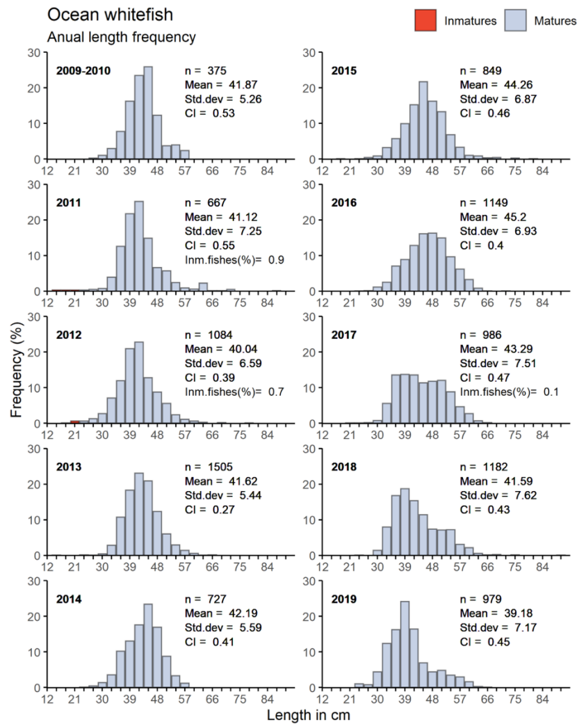
Figure 78. [CA13]Length-frequency data for pierna aggregated across all years (2009-2019) and depth categories; plotted by time period. Size at maturity according to Ramirez-Luna (2010).
