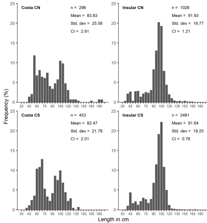
Figure 60. Length-frequency data of jurel aggregated across all years (2009-2019); plotted by coastal (costera) and offshore (Insular) in the north and south of El Corredor.
