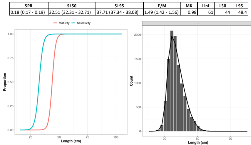
Figure 39. Initial LBSPR assessment of pargo amarillo using size composition of the catch data aggregated across all years, fishing areas and depths; assuming L_{\infty} = 61 cm & L_m/L_{\infty} = 0.72 to infer L_{50} = 44 cm. The table shows derived estimates of spawning ratio potential (SPR) and the size of 50% and 95% selectivity (SL50 & SL95) and relative fishing pressure (F/M). The estimated 95% confidence intervals around these mean estimates are shown in brackets. The input parameters assumed are indicated to the right; life history ratio M/K, asymptotic size (Linf), size at 50% and 95% maturity (L50 & L95). The left-hand panel presents plots of assumed size of maturity ogive (red) and the estimate size of selectivity (blue). The right-hand panel plots the size composition data analysed (black bars) and the LBSPR modelled fit to those data.
