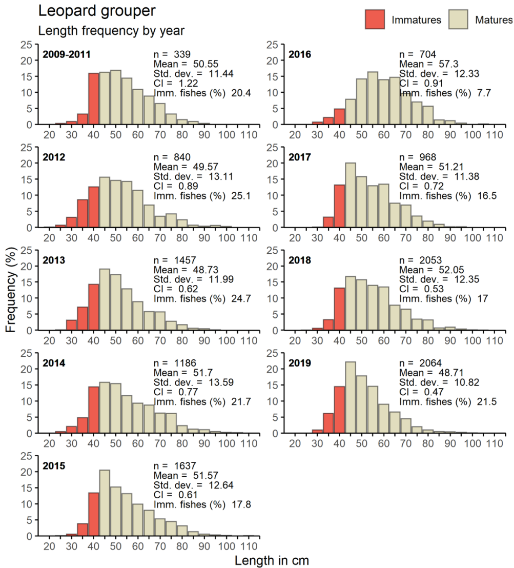
Figure 20. Length-frequency data for cabrilla sardinera aggregated across all years (2009-2019) and depth categories; plotted by time period. Size at maturity according to Perez-Olivas et al. (2018) indicated by darker colouring.
