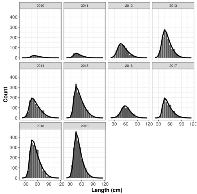
Figure 28. Initial LBSPR assessment of cabrilla sardinera using size composition of the catch data aggregated fishing areas and depths and fitted by year. Plots of the size composition data analysed (black bars) and the LBSPR modelled fit to those data (black line).
