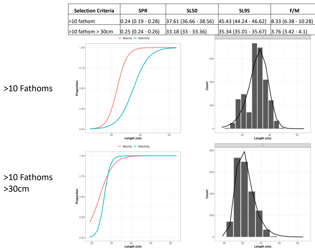
Figure 109. Initial LBSPR assessments using size composition of the catch data aggregated for 2017 - 2020, and fishing areas from depths \geq 10 fathoms (upper panel), and (lower panel) truncated at 30 cm. The table shows derived estimates of spawning ratio potential (SPR) and the size of 50% and 95% selectivity (SL 50 & SL 95 ) and relative fishing pressure (F/M). The estimated 95% confidence intervals around these mean estimates are shown in brackets. The input parameters assumed are indicated to the right; life history ratio M/K, asymptotic size (L ∞ ), size at 50% and 95% maturity (L 50 & L 95 ). The left-hand panels present plots of assumed size of maturity ogive (red) and the estimate size of selectivity (blue). The right-hand panels plot the size composition data analysed (black bars) and the LBSPR modelled fit to those data
