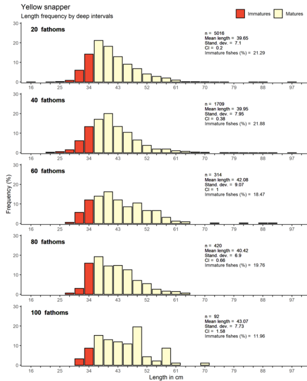
Figure 32. Length-frequency data aggregated across all years (2009-2019) and all fishing locations plotted by depth category. Size at maturity according to Barbosa-Ortega et al. (2014) indicated by darker colouring.
