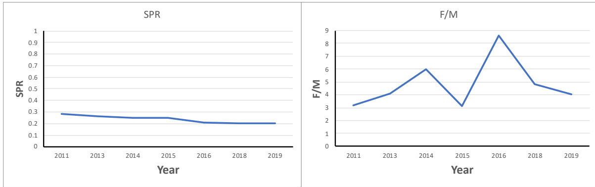
Figure 71. Initial annual LBSPR assessment of jurel using size composition of the catch aggregated across fishing areas from \geq 40 fathoms and truncated at 75 cm; assuming L_{\infty} = 153 cm & L_m/L_{\infty} = 0.72 to infer L_{50} = 95 cm. Plots of the estimate trend in SPR (left) and relative fishing pressure (F/M) by year (right).
