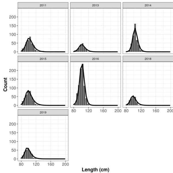
Figure 70. Initial annual LBSPR assessment of jurel using size composition of the catch aggregated across fishing areas from \geq 40 fathoms and truncated at 75 cm; assuming L_{\infty} = 153 cm & L_m/L_{\infty} = 0.72 to infer L_{50} = 95 cm. Plots of the size composition data analysed (black bars) and the LBSPR modelled fit to those data (black line).
