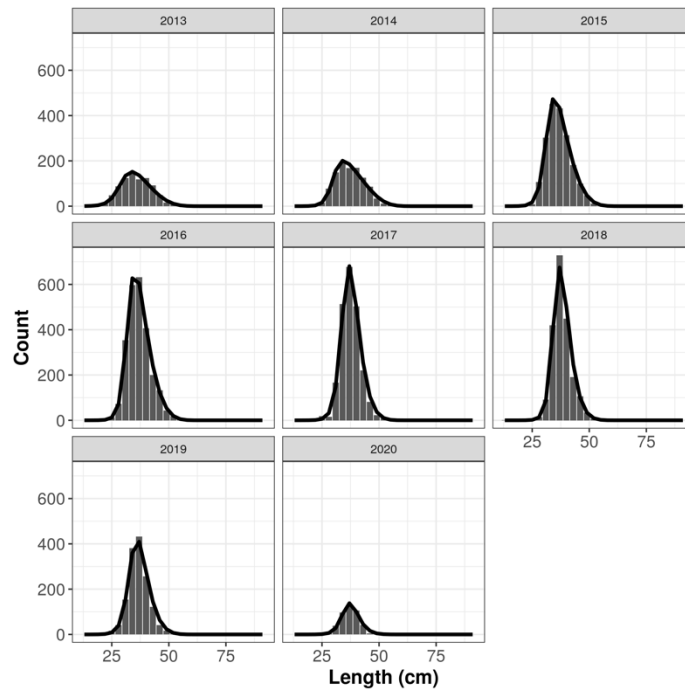
Figure 15. Initial LBSPR assessment of cochito using size composition of the catch data aggregated fishing areas and depths and fitted by year, assuming Monocanthidae LHR ( M/k=1.47 ; L_m/L_\infty = 0.647 ) and L_m = 33.5 cm as estimated for El Corredor and thus L_\infty = 52 cm. Plots of the size composition data analysed (black bars) and the LBSPR modelled fit to those data (black line).
