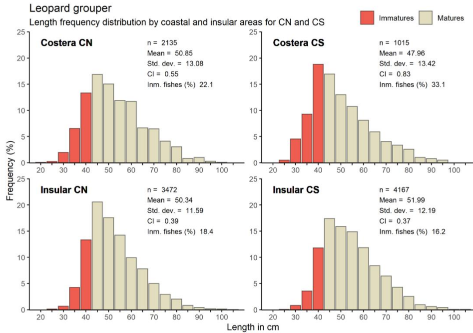
Figure 18. Length-frequency data for cabrilla sardinera aggregated across all years (2009-2019); plotted by coastal (costera) and offshore (Insular) in the north and south of El Corredor. Size at maturity according to Perez-Olivas et al. (2018) indicated by darker colouring.
