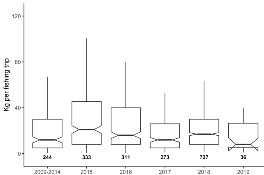
Figure 7. Catch-Per-Unit-Effort data for cochito aggregated across all depth categories and fishing areas, plotted annually or time period. Bold values mark sample size for depth category, black horizontal bars indicate medians with 95% confidence intervals indicated by notches, boxes indicate interquartile range (0.25 – 0.75) and vertical lines the range. The unusual shape of the last boxplot indicates the low sample size.
