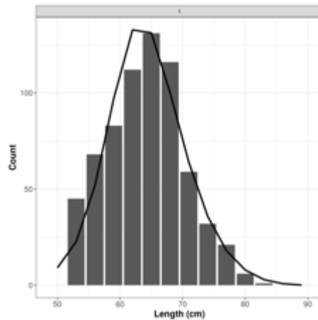
Figure 101. LBSPR fitting to the huachinango catch size composition data from 2019 and 2019 from 60 and 80 fathoms and truncated to exclude TL < 54cm.
