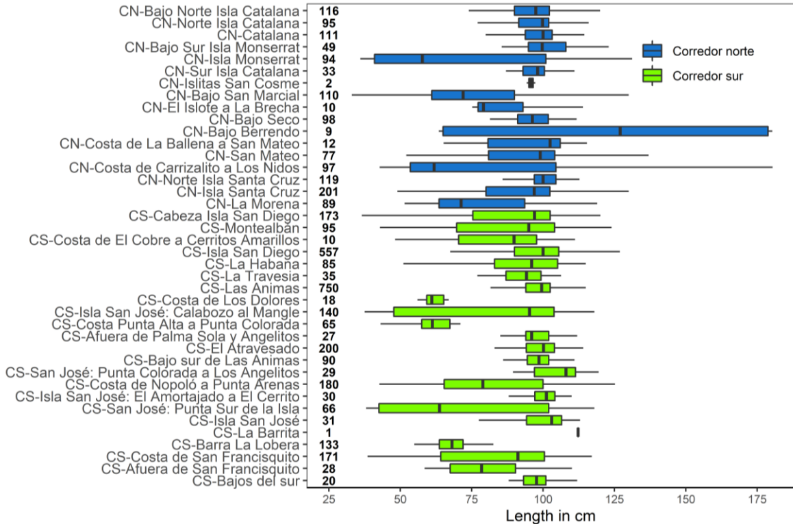
Figure 59. Percentile length-frequency data for jurel aggregated across all years (2009-2019) and depth categories; plotted by fishing areas sorted north to south. Bold values mark sample size for each area, black bars indicate median, coloured bars indicate interquartile range (0.25 – 0.75), horizontal lines the range. Confidence intervals cannot be estimated due to low record numbers for most fishing areas.
