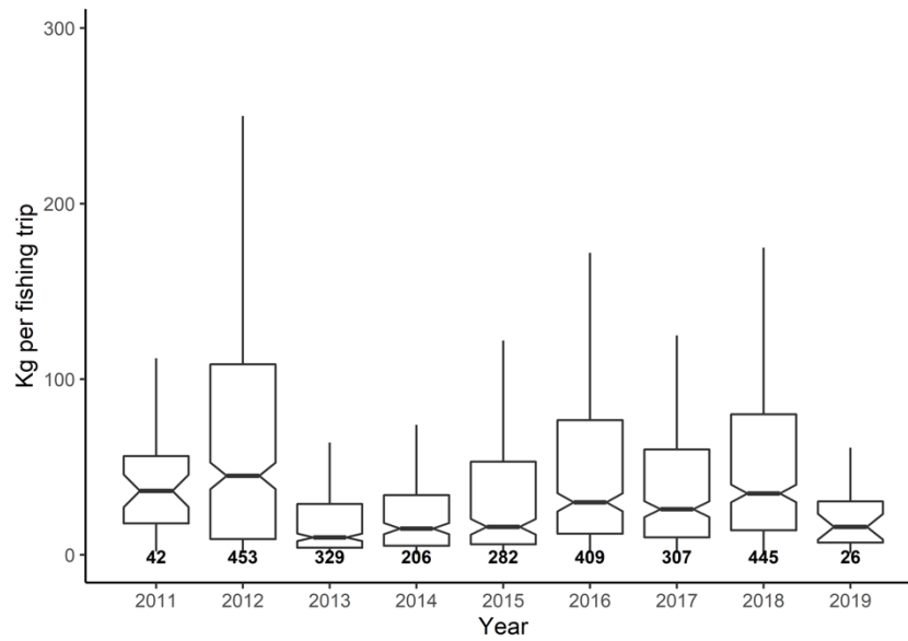
Figure 81. Catch-Per-Unit-Effort data for pierna aggregated across all fishing grounds and depth categories; plotted by year. Bold values mark sample size for depth category, black horizontal bars indicate medians with 95% confidence intervals indicated by notches, boxes indicate interquartile range (0.25 – 0.75) and vertical lines the range.
