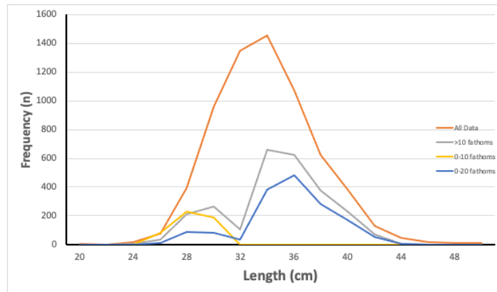
Figure 102. Various aggregations and subsets of verdillo length-frequency data; all data 2010-2020, 0-10 fathoms 2017-20 (scaled up by 10 x), 0-20 fathoms 2017-20 and > 10 fathoms 2017-20.
