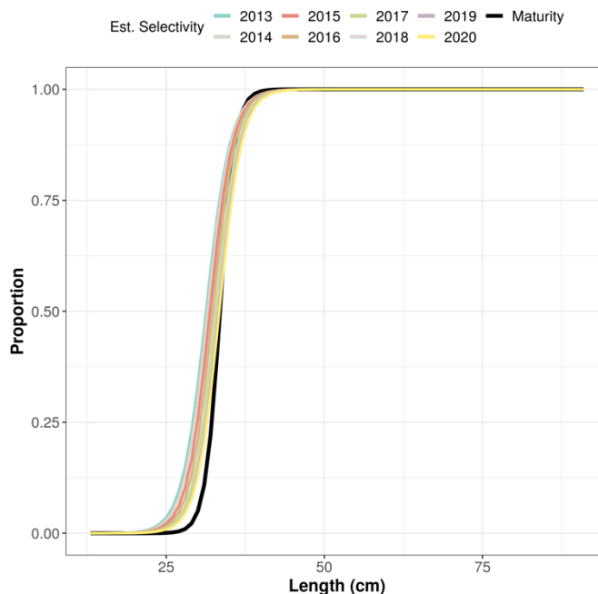
Figure 14. Results of initial LBSPR of cochito using size composition of the catch data aggregated fishing areas and depths and fitted by year, assuming Monocanthidae LHR ( M/k=1.47 ; L_m/L_{\infty} = 0.647 ) and L_m = 33.5 cm as estimated for the Corridor and thus L_{\infty} = 52 cm. Plots of assumed size of maturity ogive (black) and estimated size of selectivity (coloured).
