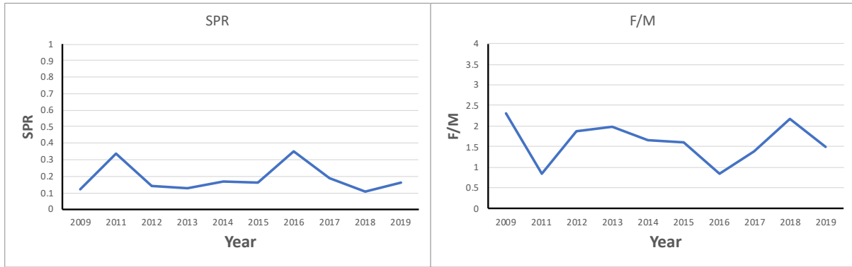
Figure 42. Initial LBSPR assessment of pargo amarillo using size composition of the catch data aggregated fishing areas and depths and fitted by year, assuming L_{\infty} = 61 cm & L_m/L_{\infty} = 0.72 to infer L_{50} = 44 cm. Plots of the estimate trend in SPR (left) and relative fishing pressure (F/M) by year (right).
