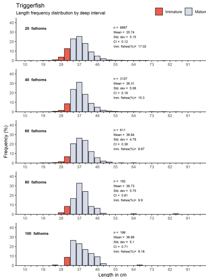
Figure 3. Length-frequency data for cochito aggregated across all years (2009-2019) and fishing locations; plotted by depth category. Size at maturity (33.8 cm) according to Camacho Mondragon et al. (2019) indicated by darker colouring.
