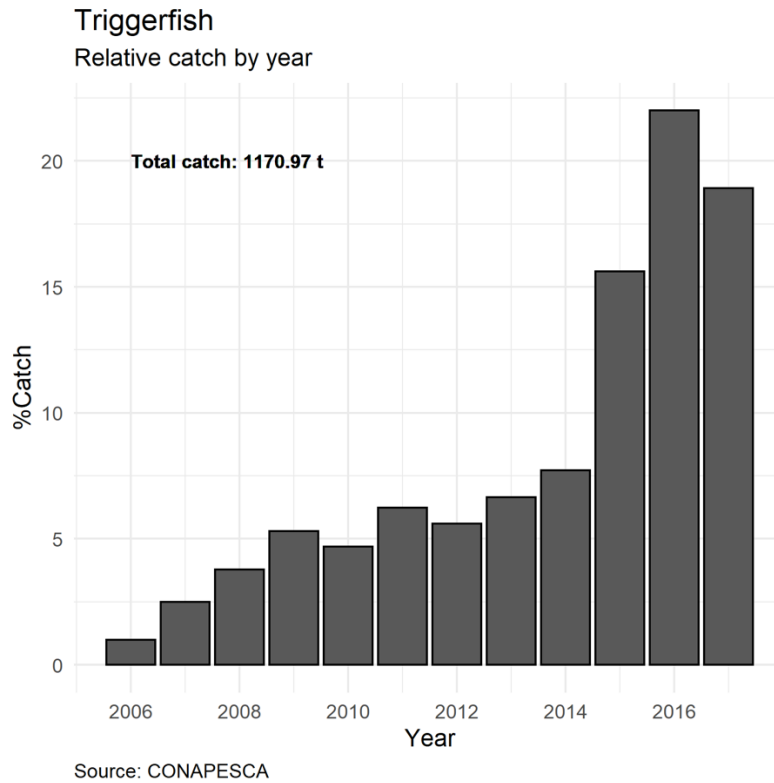
Figure 8. The proportion of total recorded catch of cochito from 2006-2017 (1170.97t) that was recorded in each year of that time series. This figure shows that >50% of the recorded cochito catch was taken in the final three years of the time series.
