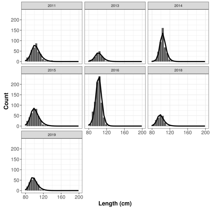
Figure 73. Annual LBSPR assessment of jurel using size composition of the catch aggregated across fishing areas from \geq 40 fathoms and truncated at 75 cm; assuming L_{50} = 90 cm & L_m/L_\infty = 0.72 to infer L_\infty = 145 cm. Plots of the size composition data analysed (black bars) and the LBSPR modelled fit to those data (black line).
