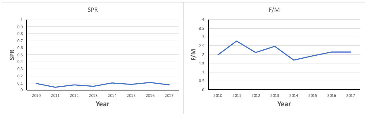
Figure 29. Initial LBSPR assessment of cabrilla sardinera using size composition of the catch data aggregated fishing areas and depths and fitted by year. Plots of the estimate trend in SPR (left) and relative fishing pressure (F/M) by year (right).
