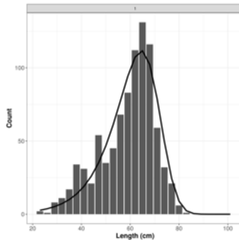
Figure 100. LBSPR fitting to the huachinango catch size composition data from 2019 and 2020 from \geq 60 fathoms.
