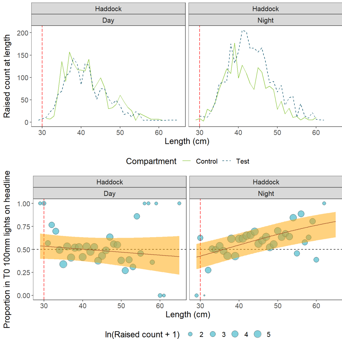
Figure 3. Length frequency distributions (LFD) (top) and catch curves (bottom) for haddock. Navy hatched line represents the test gear and green solid line represents the control gear in the LFD plot. Overall modelled proportions of haddock catch at length in the test gear are outlined in the catch curves by day and night. Points represent the empirical raised proportions over all hauls with point sizes proportional to the raised counts. Model fit and 95% confidence intervals (yellow band) come from the GAM. Vertical lines represent the minimum conservation reference size for haddock ( \geq 30 cm).
