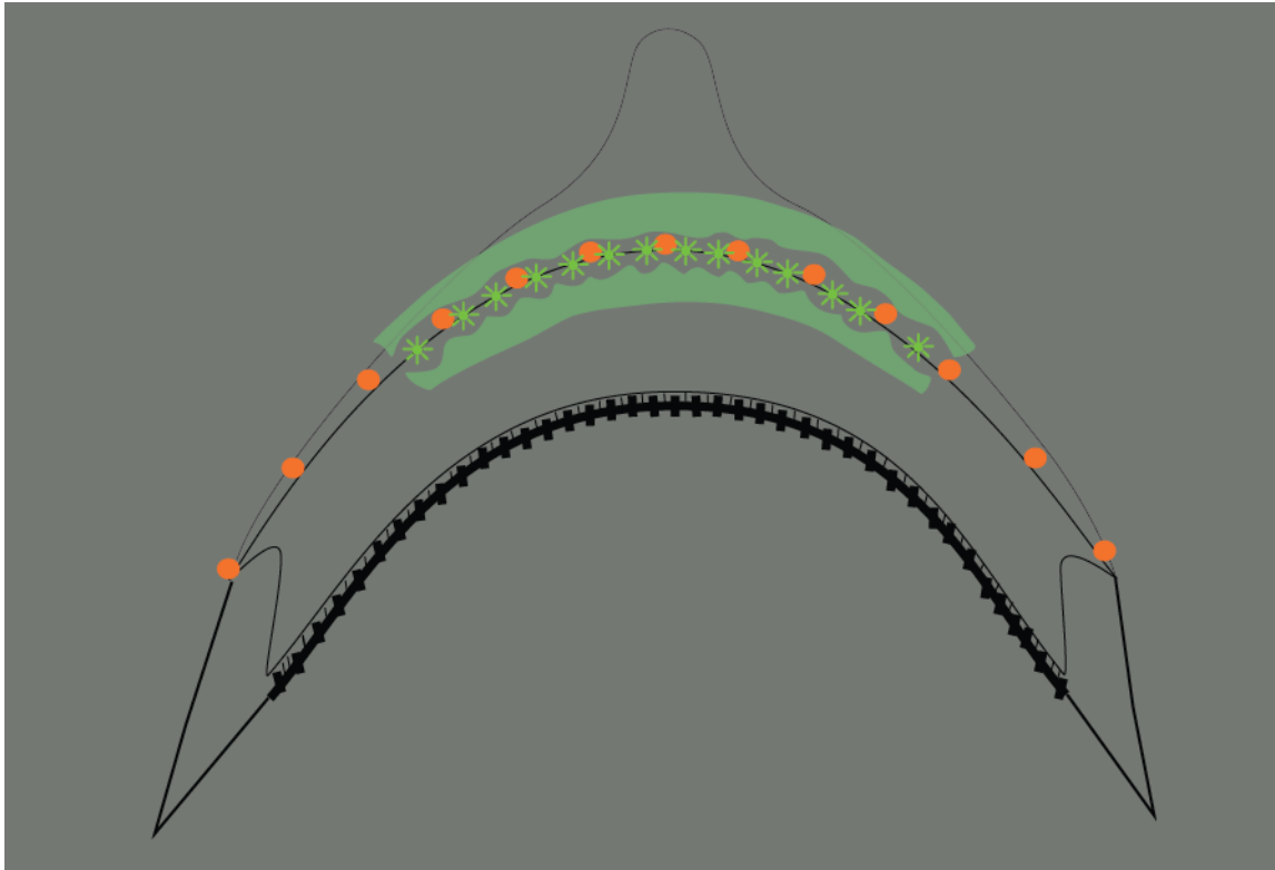
Figure 2. Trawl with 14 green artificial lights on the headline
