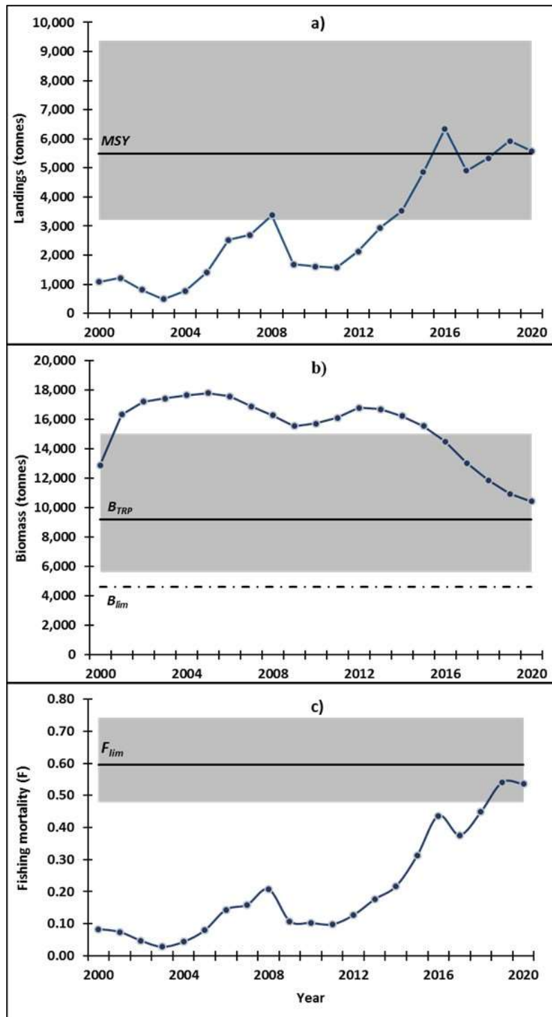
Figure 10.- Results of the C-MSY method for management purposes based on Monte Carlo assessment for the cuota swimcrab ( Callinectes arcuatus ) stock from the Gulf of California (CC_GC): a) landings, MSY with 95% confidence interval (gray area) b) Biomass trajectory, TRP_{BMSY} with 95% confidence interval (gray area) and LRP_{BMSY} . (Dotted line) c) Fishing mortality and LRP_{FMSY} with 95% confidence intervals (gray area).
