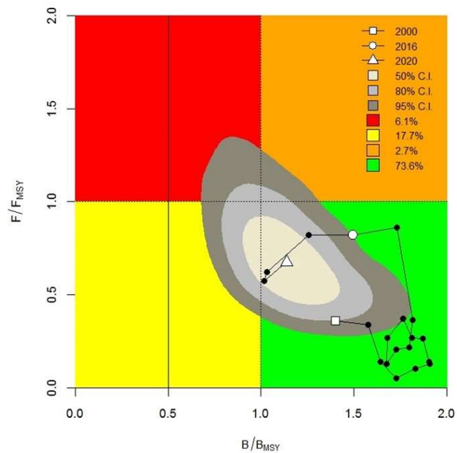
Figure 14.- Kobe plot for the warrior swimcrab fishery (WC_BC) of the west coast of Baja California. The gray areas indicate the iso-probabilities.
