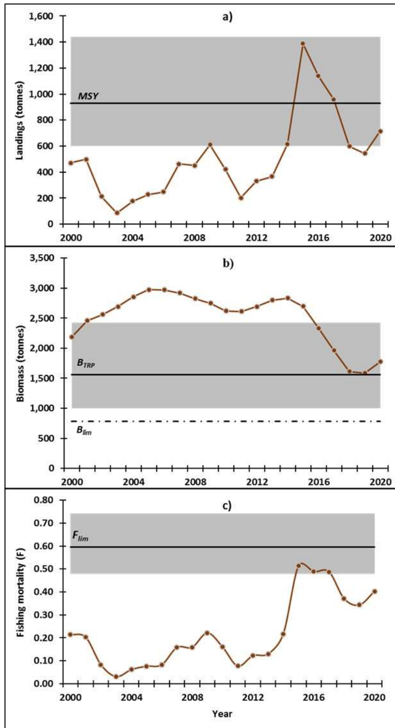
Figure 11.- Results of the C-MSY method for management purposes based on Monte Carlo assessment for the warrior swimcrab ( Callinectes bellicosus ) stock from west coast of Baja California, México (WC_BC): a) landings, MSY with 95% confidence interval (gray area) b) Biomass trajectory, TRP BMSY with 95% confidence interval (gray area) and LRP BMSY (dotted line) c) Fishing mortality and LRP FMSY with 95% confidence intervals (gray area).
