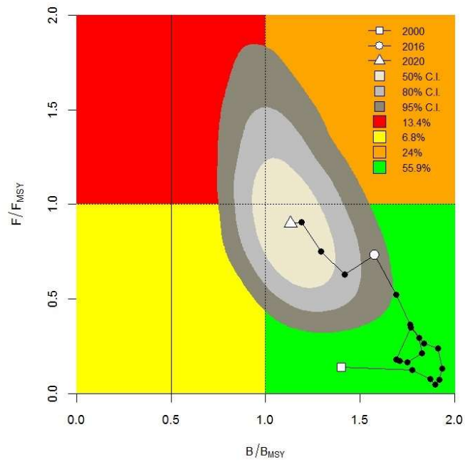
Figure 13.- Kobe plot for the cuota swimcrab fishery (CC_GC) in the Gulf of California, Mexico. Gray areas indicate iso-probabilities.
