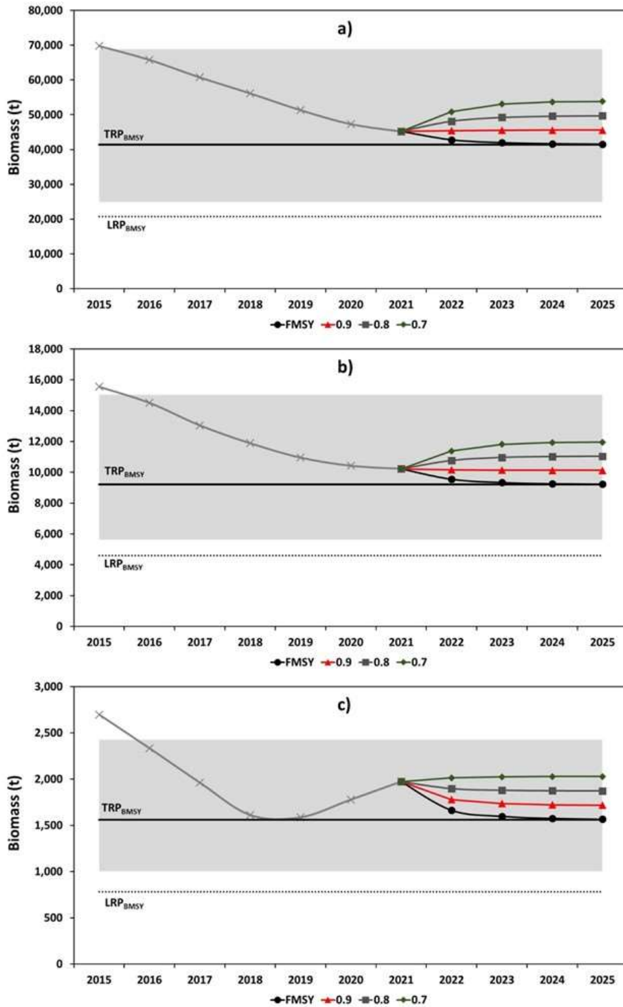
Figure 16.- Standard management scenarios projected to 2025 for the swimcrabs stocks, using fishing mortality as the management parameter, including LRP_{FMSY} and three lesser F values. a) WC_GC, b) CC_GC and c) WC_BC. The solid lines show TRP_{BMSY} . The dotted lines show LRP_{BMSY} . The gray area show confidence intervals of B_{MSY} . Refer to Figures 11b, 12b and 13b respectively to view the historic biomass trajectory (gray line).
