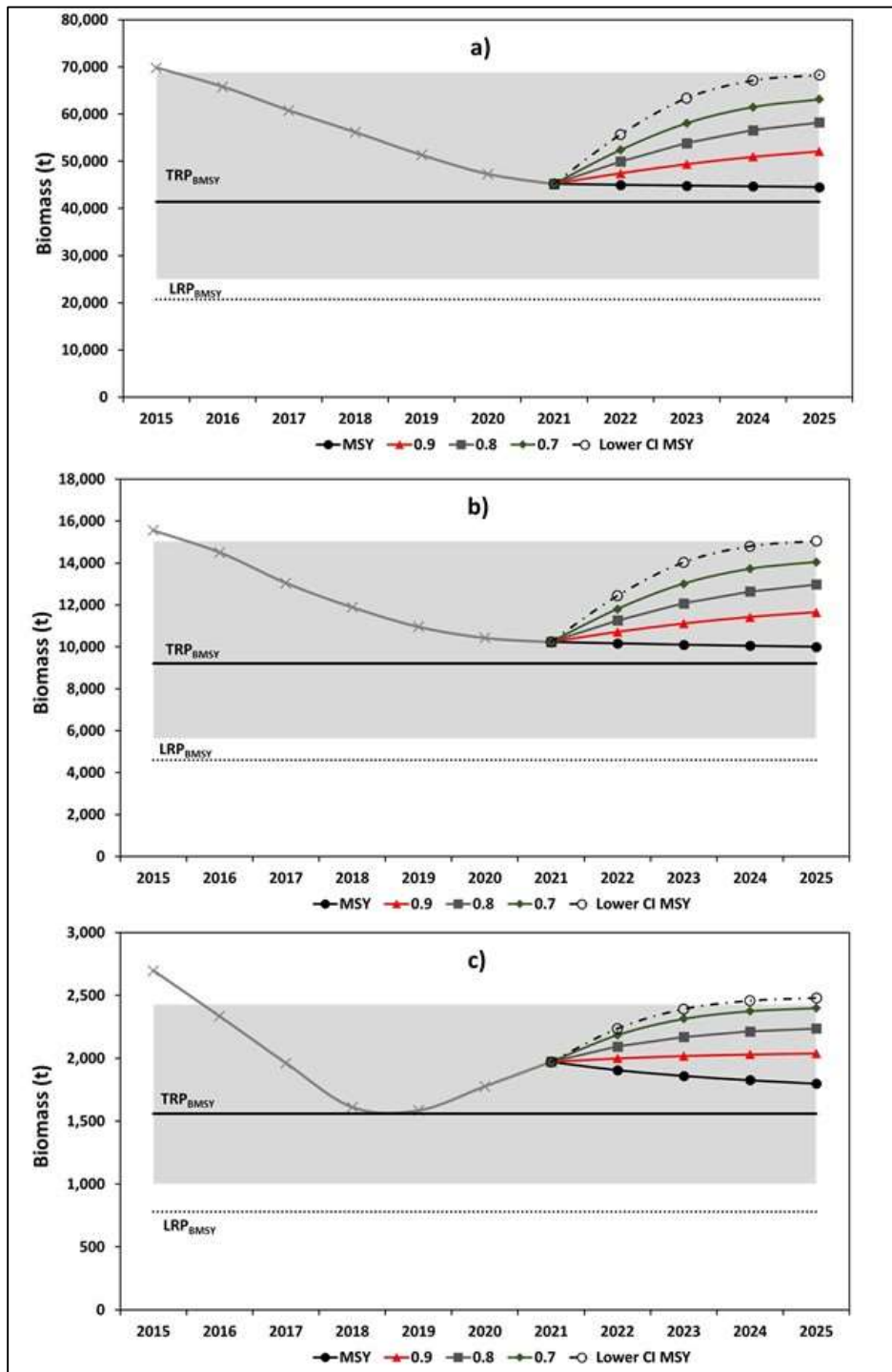
Figure 15.- Standard management scenarios projected to 2025 for the swimcrabs stocks, using harvest value as the management parameter, including the MSY and lower confidence interval of MSY as well as values in between. a) WC_GC, b) CC_GC and c) WC_BC. The solid lines show TRP_{BMSY} . The dotted lines show LRP_{BMSY} . The gray area show confidence intervals of B_{MSY} . Refer to Figures 11b, 12b and 13b respectively to view the historic biomass trajectory (gray line).
