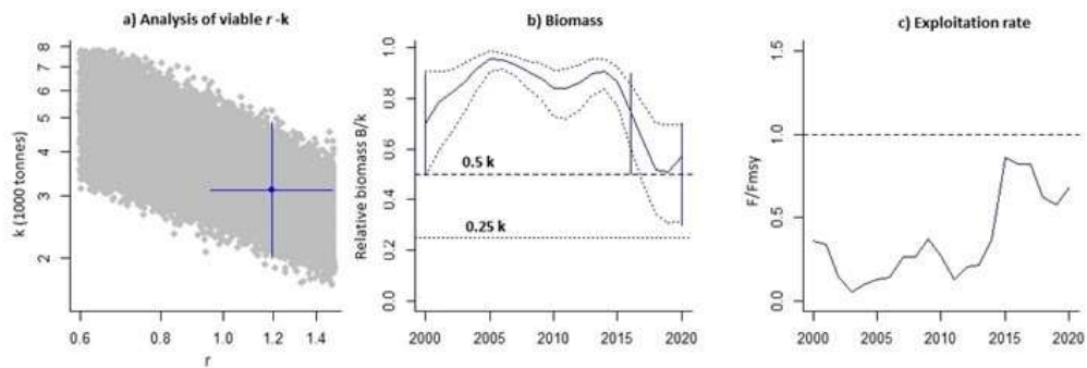
Figure 5.- Results of the C-MSY method for the warrior swimcrab stock off the west coast of Baja California (WC_BC). a) Analysis of the most probable combinations of r and k . The viable r - k pairs that fulfilled conditions are shown in grey. The blue cross, with approximate 95% confidence limits, marks the most probable r - k pair. b) Biomass relative to the size of the population carrying capacity in the time analyzed with 2.5 and 97.5 percentiles. c) Exploitation rate of the stock.
