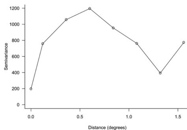
Fig. 2. Semivariogram analysis of the abundances (CPUA; Org. km -2 ) of the red octopus ( Octopus maya ) in the north-eastern Campeche Bank, Mexico. The behaviour indicated a grouped type distribution.
